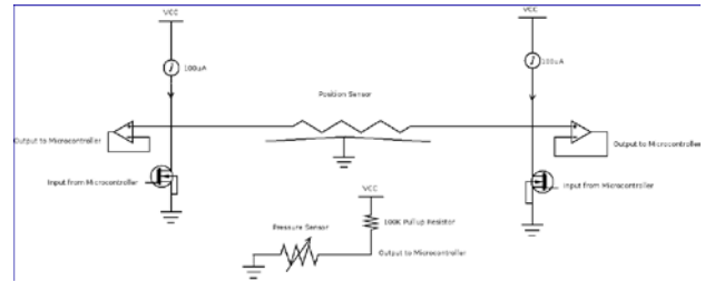
Figure 7 Analog Front-end
