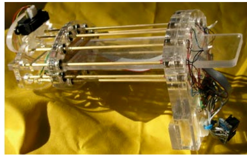
Figure 2. Rotating Rods (12)
